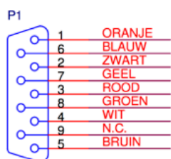
CONNECTOR DB9
